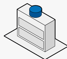
➤ Suction wall with the 1 st stage of filtration in corrugated cardboard and the 2 nd stage of filtration in fiber glass
