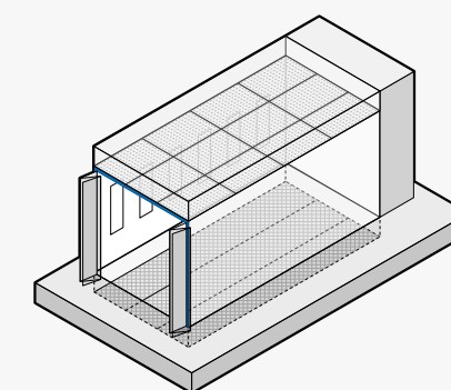
➤ Pressurised spray booth with filtered air inlet plenum and floor extraction
