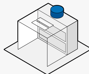
➤ Suction wall with extended walls and roof with walls and roof in galvanised sheet with lights
